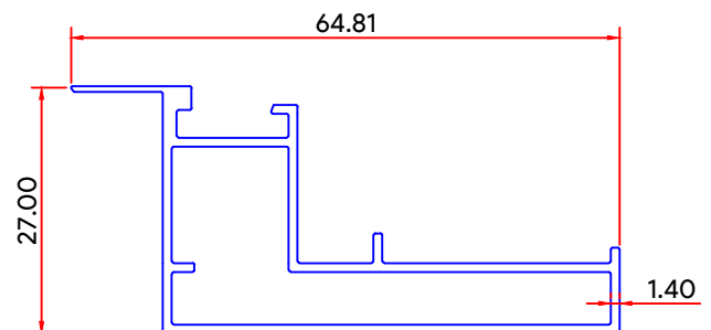
SEC. NO. : JE-255
