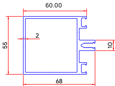
SEC. NO. : NS-35
